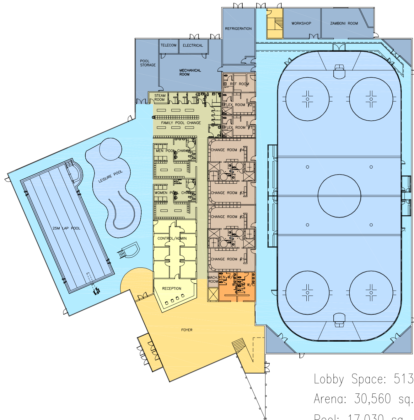
MAIN LEVEL
