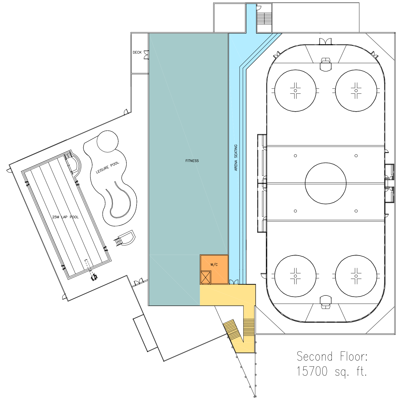
UPPER LEVEL
